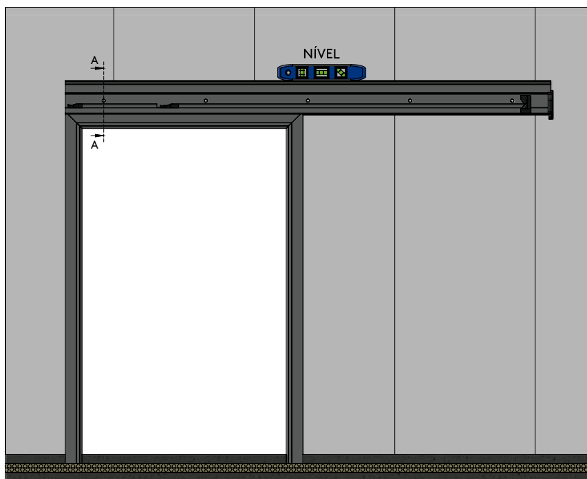
VISTA FRONTAL
